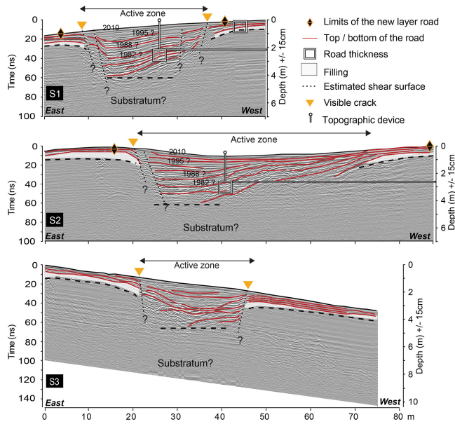
Figure 6. Interpretation of the Ground-Penetrating Radar observations for cross-sections S1, S2 and S3.
