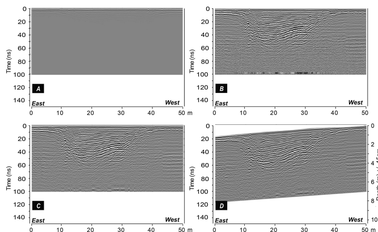
Figure 5. Illustration of the processing chain applied to the GPR observations data acquired with a 500 MHz dipole shielded antenna at profile S1. (a) Raw data, (b) processed data using gain, (c) processed data after band pass filtering, (d) conversion time-depth.
