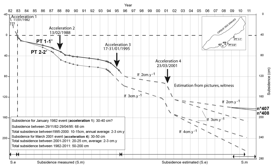
Figure 7. Subsidence of the road measured and estimated between 1982 and 2011.
