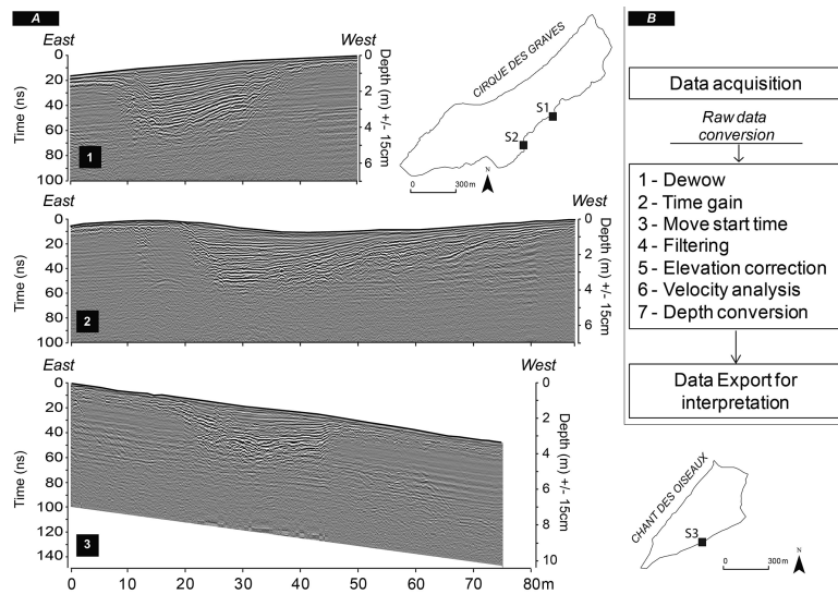
Figure 4. Example of raw GPR observations. (a) Cross-sections S1 and S2 at the “Cirque des Graves” landslide and cross-section S3 at the “Chant des Oiseaux” landslide, (b) GPR observations processing chain.
