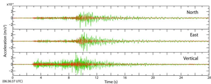
Figure 4. Comparison between waveforms of the MI=2.7 18 February 2011 Potenza earthquake recorded inside the landslide body (green curve, accelerometric station C) and on the bedrock (red curve, accelerometric station A).
