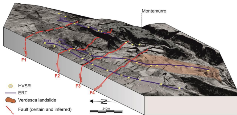
Figure 7. 3-D surface-DEM of the Montemurro area showing the faults and the location of ERT profiles and HVSR.
