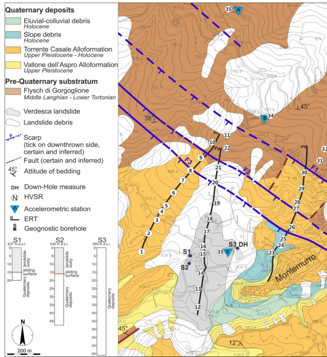
Figure 2. Simplified geological map of the study area showing the distribution of the scarp, the Verdesca landslide, the location of the surveys and the three simplified borehole logs.
